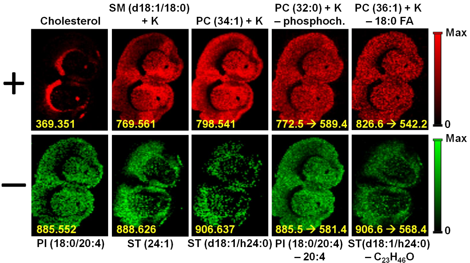
Figure 3. MS and MS/MS images for selected lipid ions. Red images are generated from positive ions, green images from negative ions. MS images are normalized to total ion count and MS/MS images are produced without any normalization.
