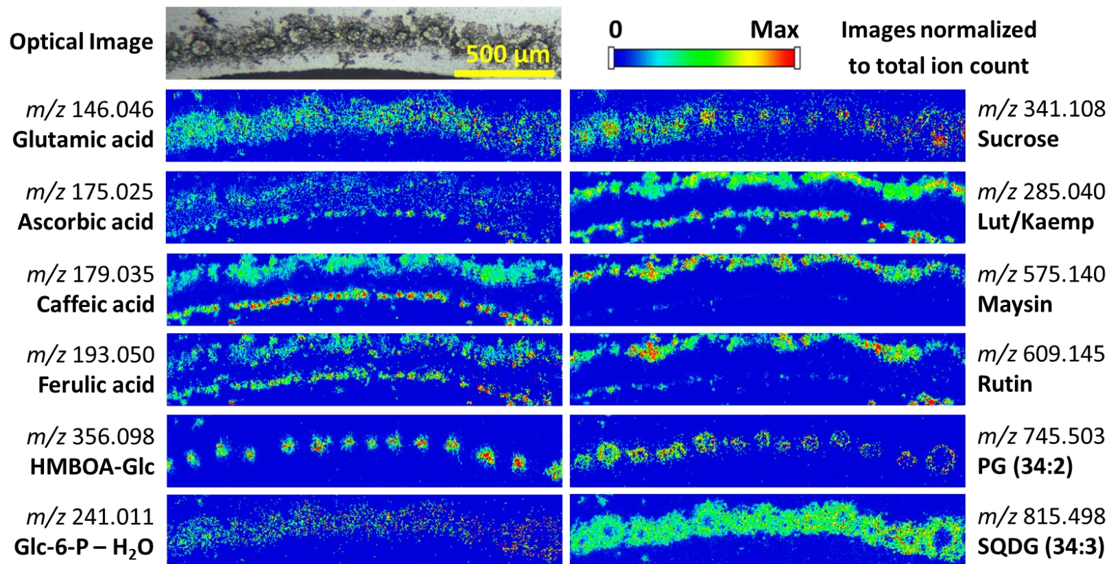
Figure 3. Optical (top left) and 5 μm raster step size MS images of various metabolites in corn leaf cross-section. Images are oriented such that the upward-facing (adaxial) surface of the leaf is at the top. HMBOA-Glc: 2-hydroxy-7-methoxy-1,4-benzoxazin-3-one; Glc-6-P: Glucose-6-phosphate; Lut/kaemp: isomeric flavonoids luteolin and kaempferol. PG: phosphatidylglycerol; SQDG: sulfoquinovosyl diacylglycerol. Signals are normalized to per-pixel TIC. Max values for generating images are as follows. Glutamic acid: 1 \times 10^{-2} . Ascorbic acid: 8 \times 10^{-3} . Caffeic acid: 3.5 \times 10^{-2} . Ferulic acid: 8 \times 10^{-3} . HMBOA-Glc: 3 \times 10^{-2} . Glc-6-P – H 2 O: 4 \times 10^{-3} . Sucrose: 6 \times 10^{-3} . Lut/kaemp: 5 \times 10^{-2} . Maysin: 5 \times 10^{-2} . Rutin: 2 \times 10^{-2} . PG (34:2): 5 \times 10^{-3} . SQDG (34:3): 3 \times 10^{-2} .
