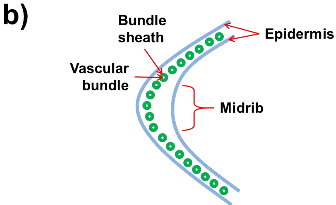
Figure S3. (a) Microscope image showing both epidermal layers, vascular bundles, bundle sheaths, and mesophyll within a transverse maize leaf section. (b) Schematic representation of the region of tissue imaged in Figure 4, showing the structures discernable from metabolite MS images.
