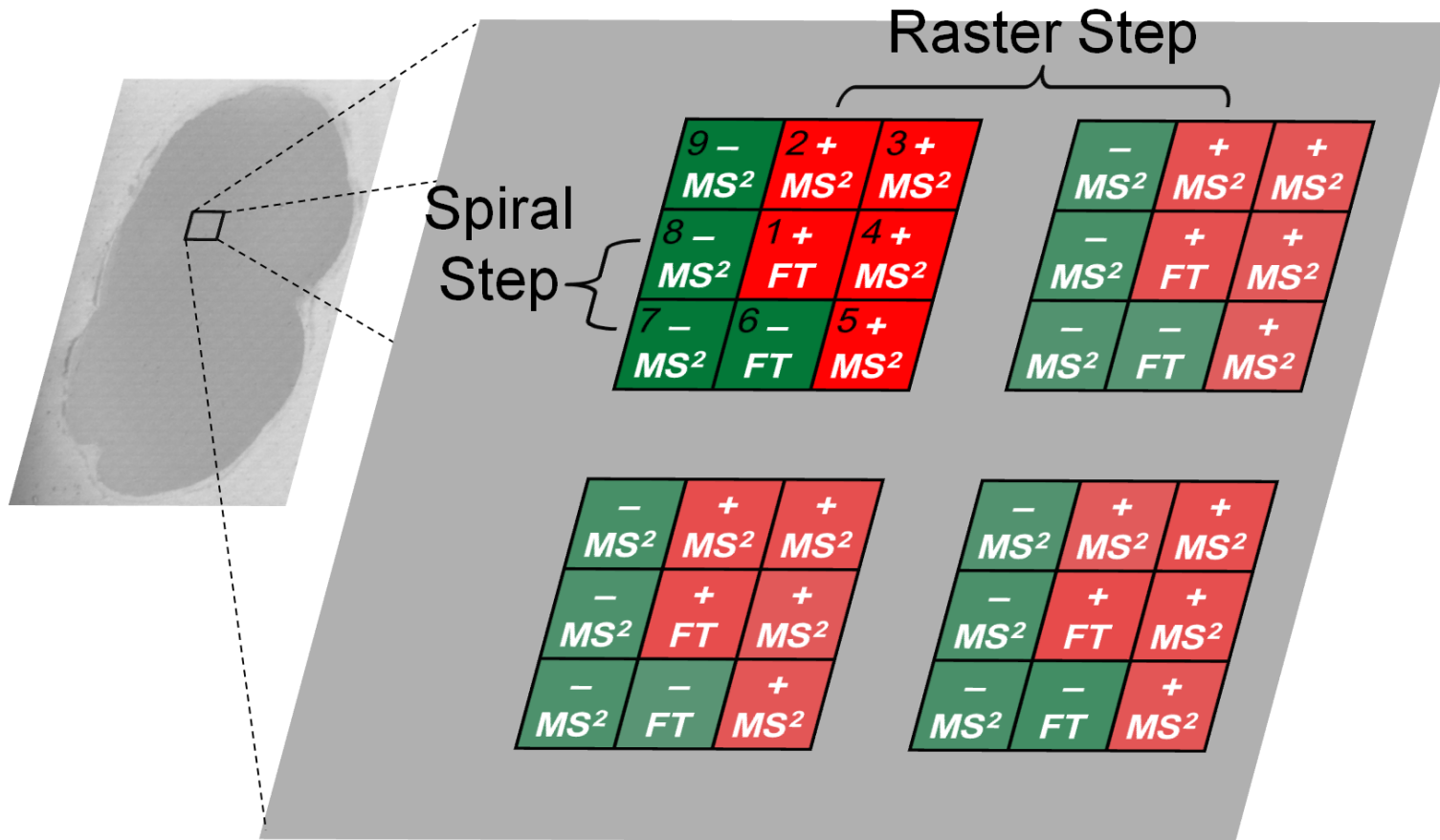
Figure 1. Illustration of spiral movement of MALDI plate and spectral acquisition method at each spiral step. The numbers indicate the order of spiral movement. A spiral step size of 25 μm (e.g. 1→2) and a raster step size of 100 μm (e.g. 1→1) were used in this experiment. FT indicates Orbitrap data acquisition. MS 2 indicates ion trap MS/MS scans. MS/MS spectra were obtained for four positive ions and three negative ions using the linear ion trap.
